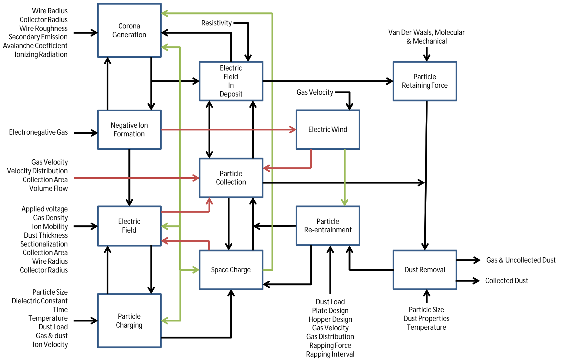
Figure 1.1. Electrostatic Precipitator System Model
